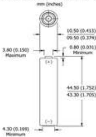
Industry Standard Dimensions
